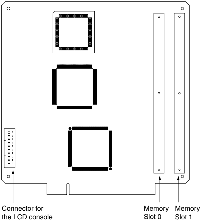
Figure 54 Layout of the CPU board
