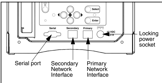
Figure 5 Network connectors
