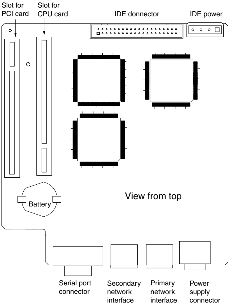
Figure 53 Layout of the input/output board
